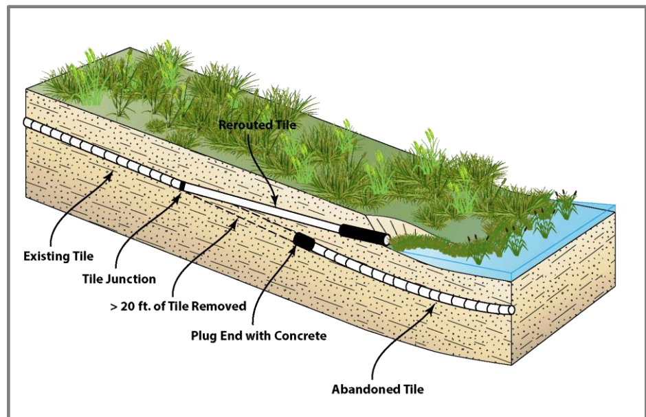
Figure 2. Modifying a Tile Drainage System to Outlet into Restored Wetland
