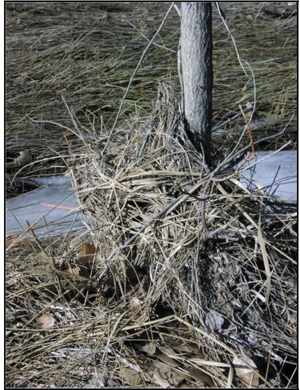
Figure 31. Drift deposit on the upstream side of a sapling in a floodplain wetland.
